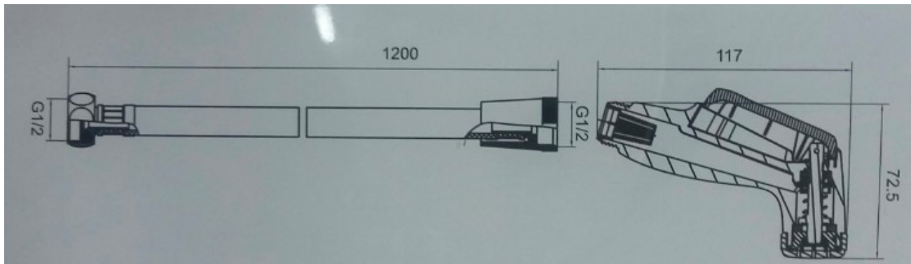
DIMENSIONAL DRAWING
